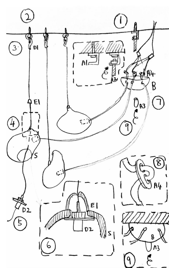
Diagram to install multiple lamps
